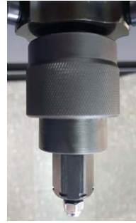
Handy depth feed locking system to prevent accidental movement of the handle during flange processing.
